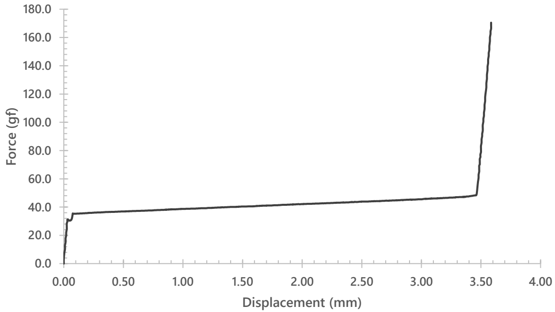
Gateron x Ukeeps Snowy Yellow Magnetic (Upstroke)
