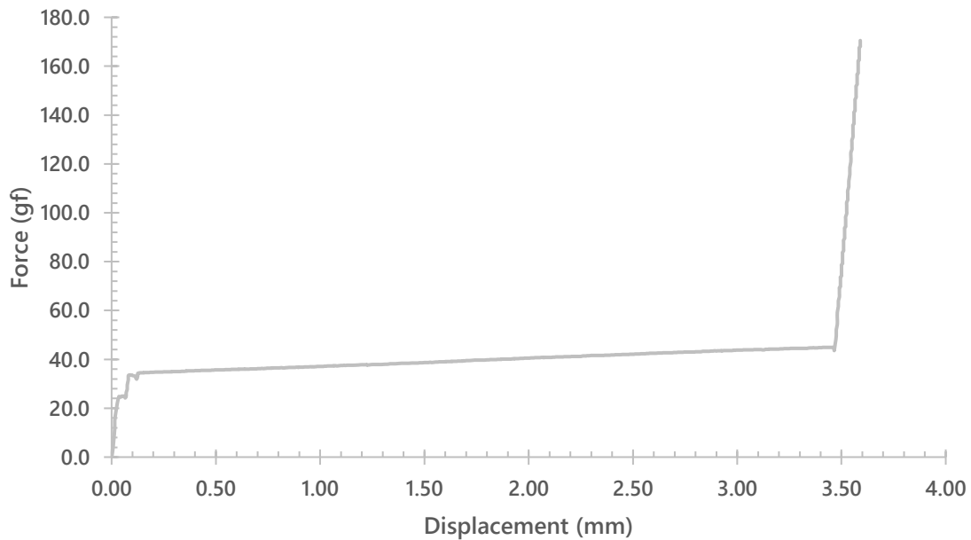
Gateron x Ukeeps Snowy Yellow Magnetic (Upstroke)
